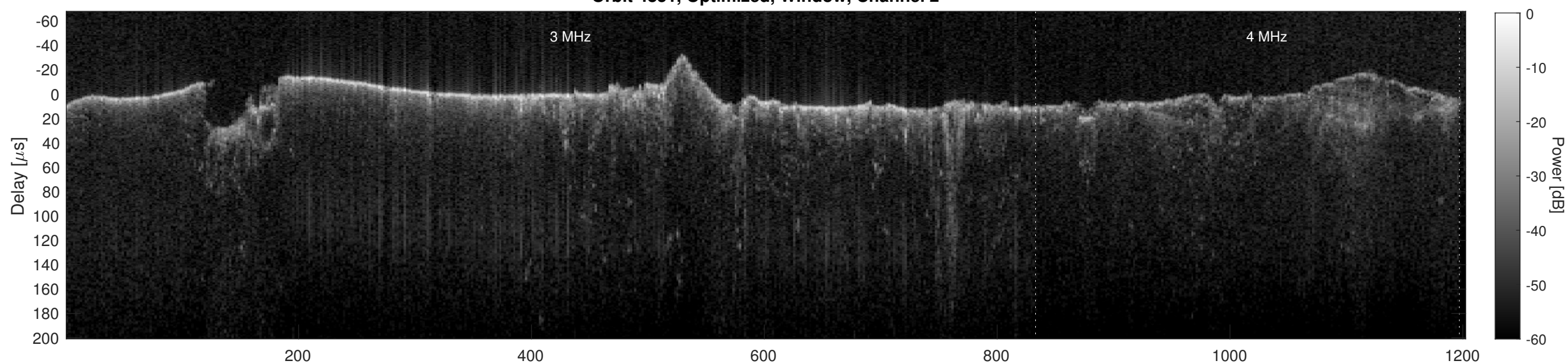
Orbit 4851, Cluttergram
