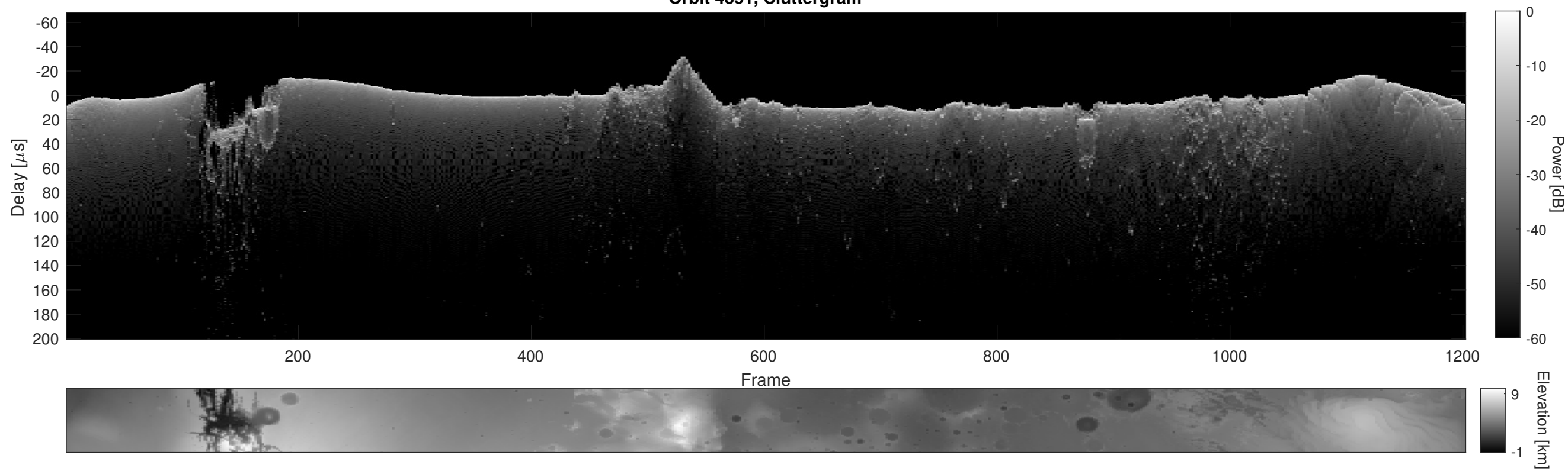
Orbit 4851, Cluttergram
