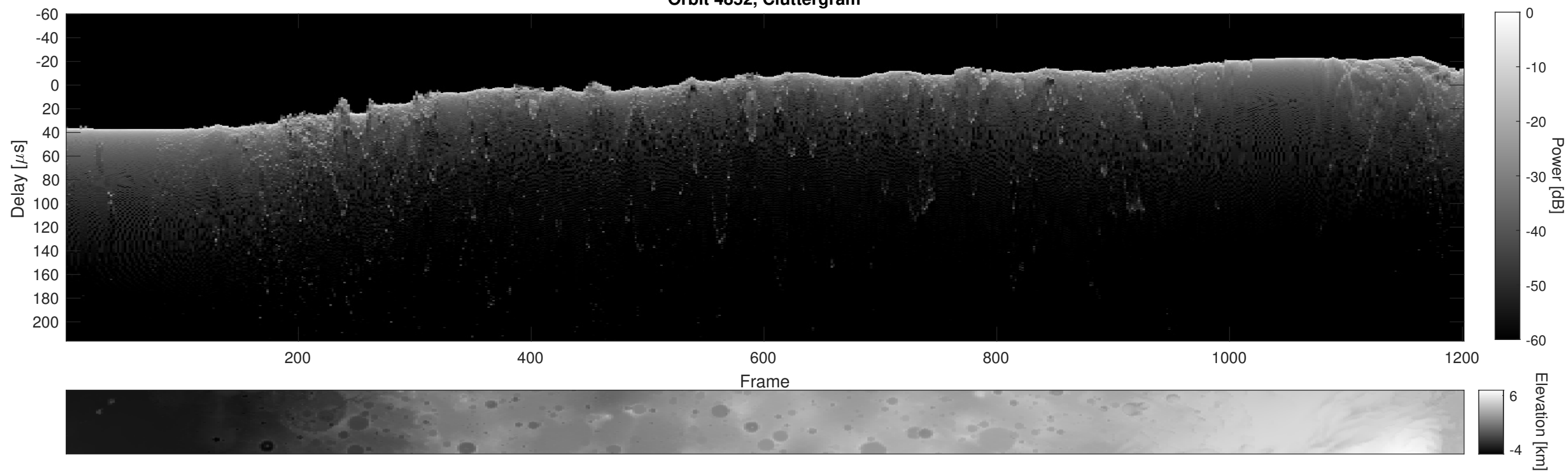
Orbit 4852, Cluttergram
