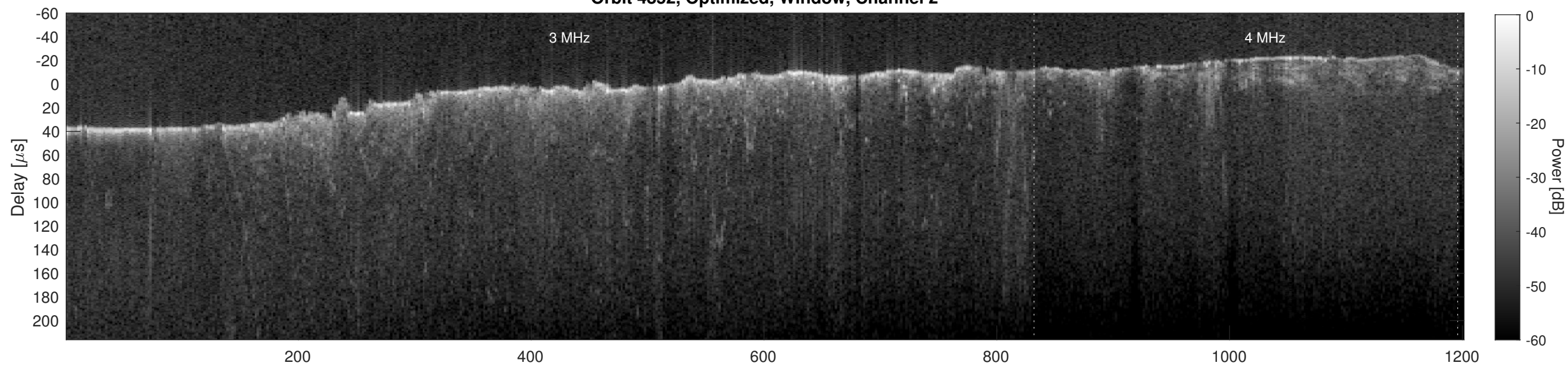
Orbit 4852, Cluttergram
