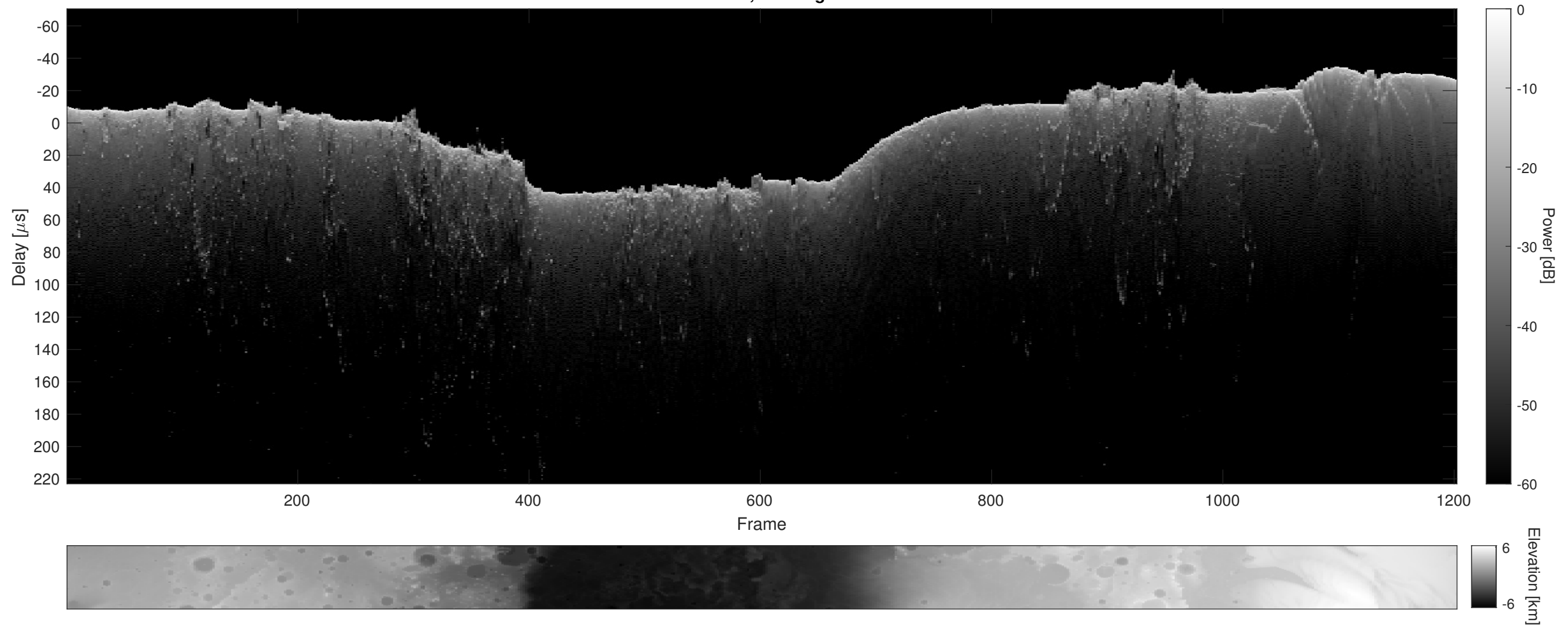
Orbit 4853, Cluttergram
