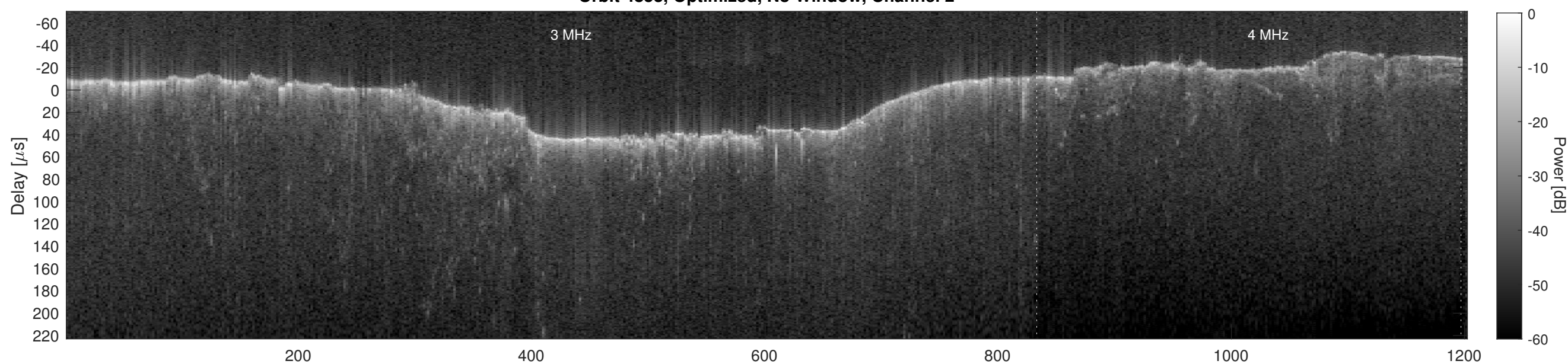
Orbit 4853, Cluttergram
