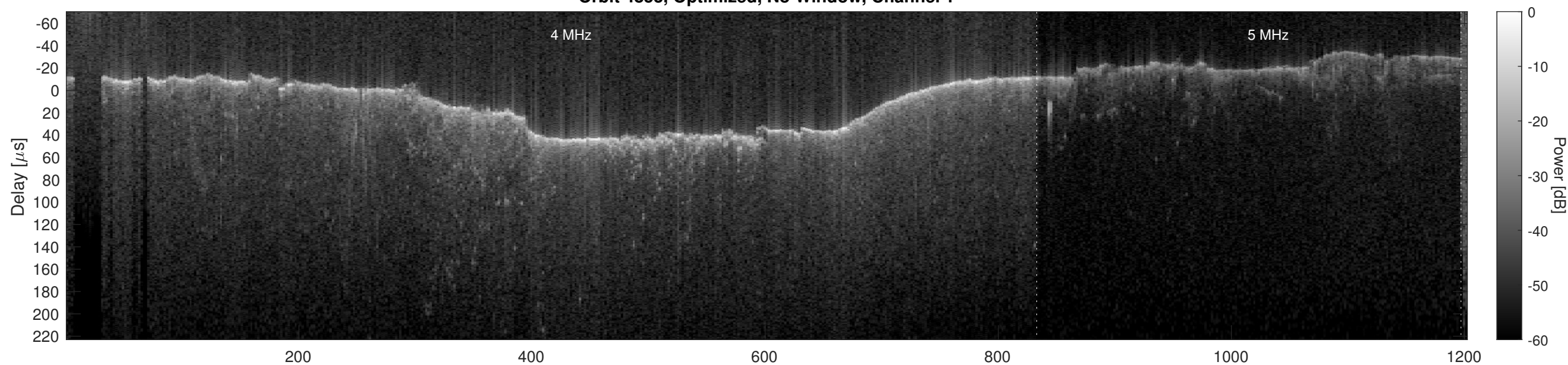
Orbit 4853, Optimized, No Window, Channel 2
