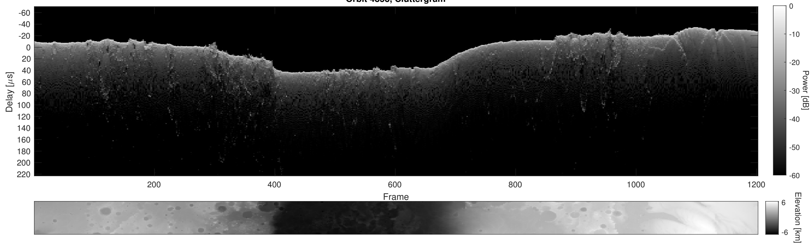
Orbit 4853, Cluttergram
