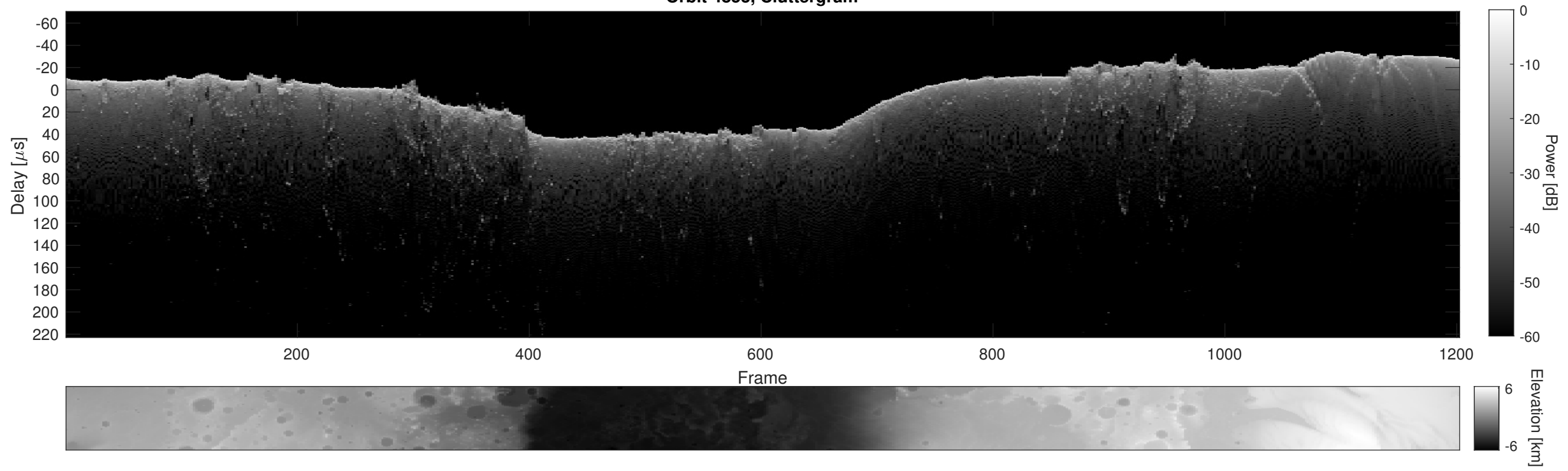
Orbit 4853, Cluttergram
