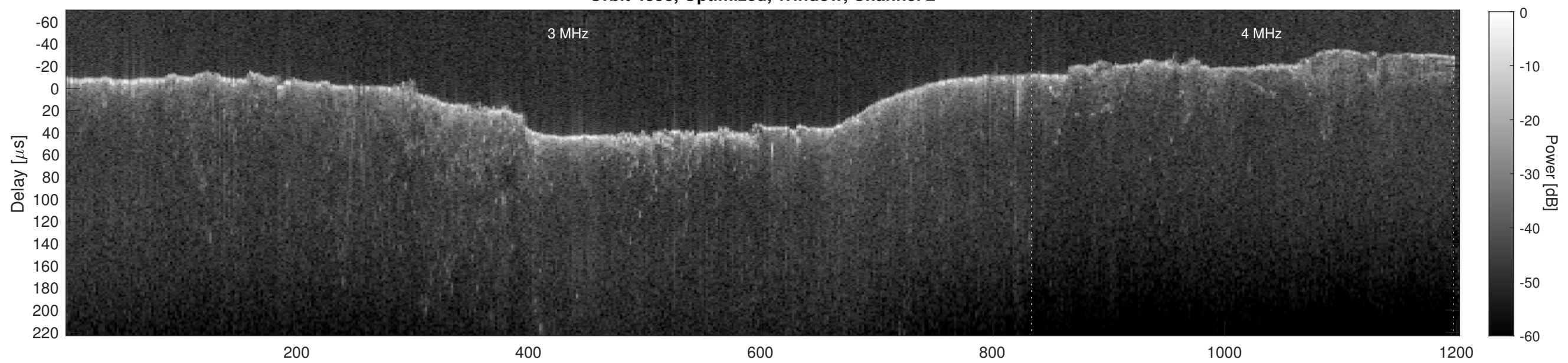
Orbit 4853, Cluttergram
