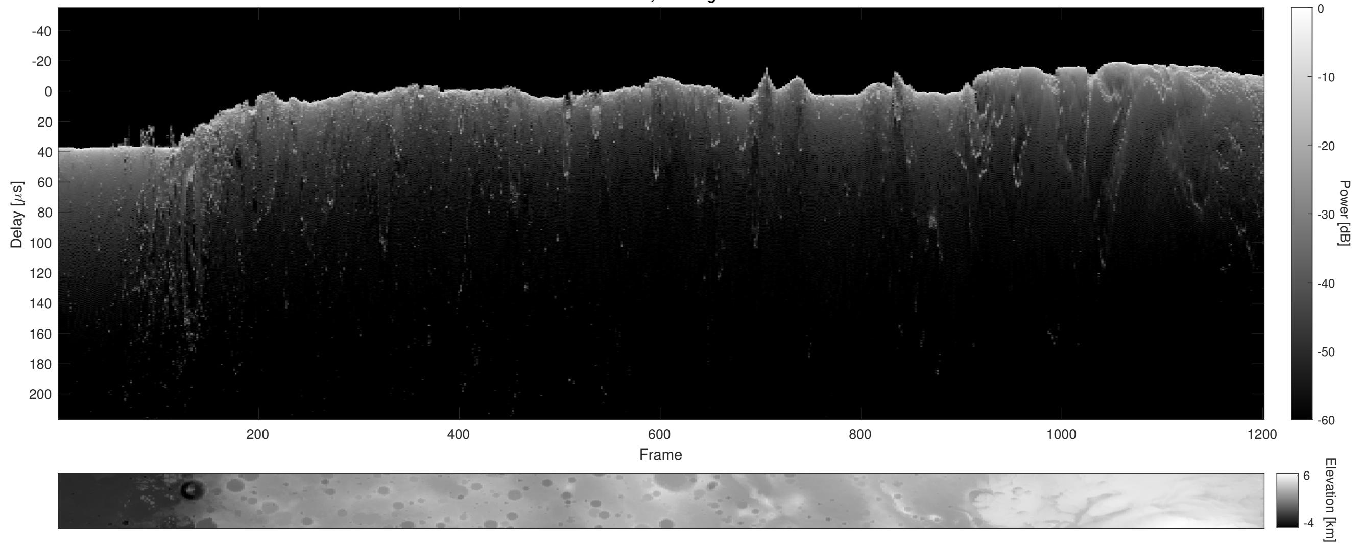
Orbit 4856, Cluttergram
