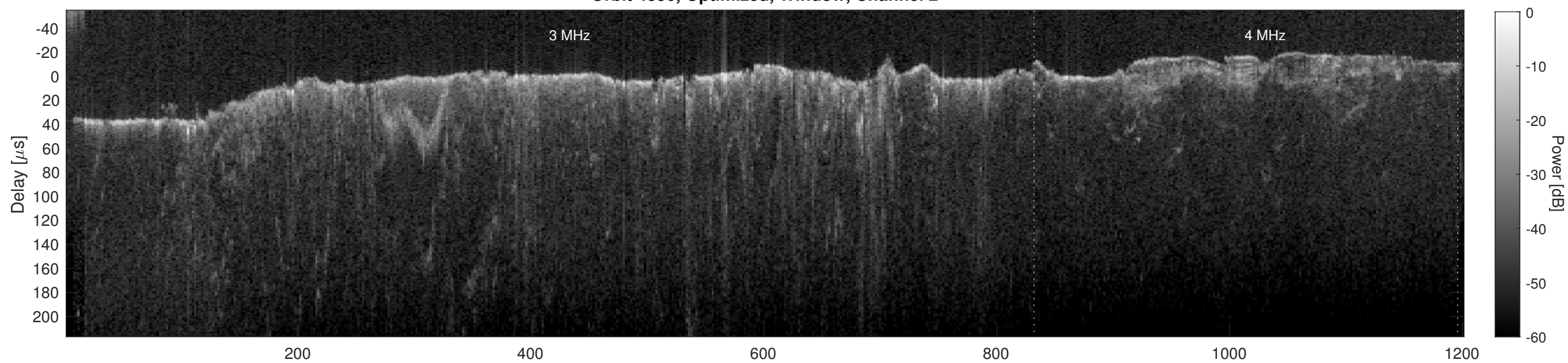
Orbit 4856, Cluttergram
