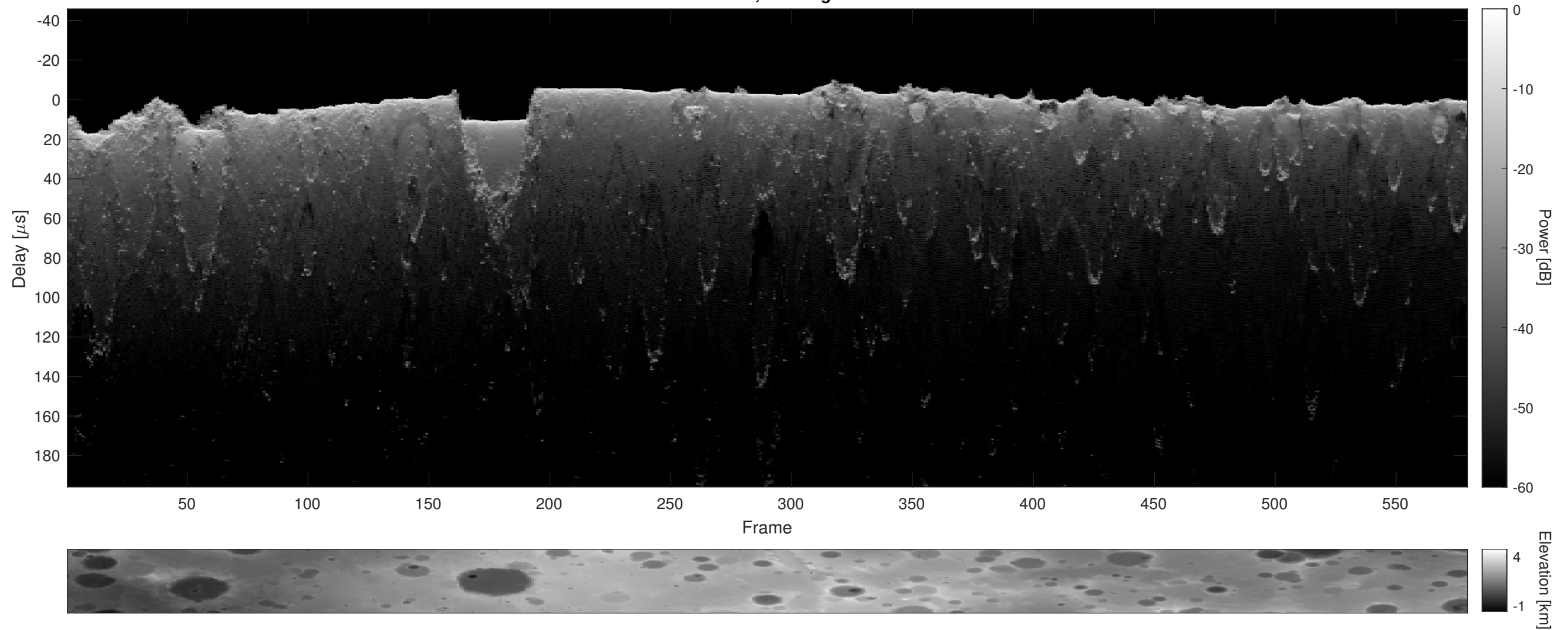
Orbit 4857, Cluttergram
