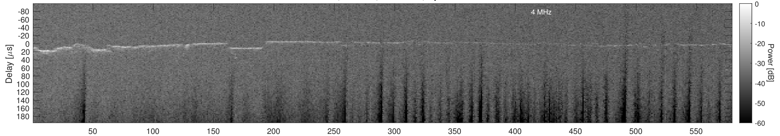
Orbit 4857, Cluttergram
