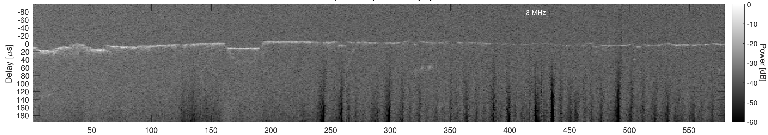
Orbit 4857, Cluttergram
