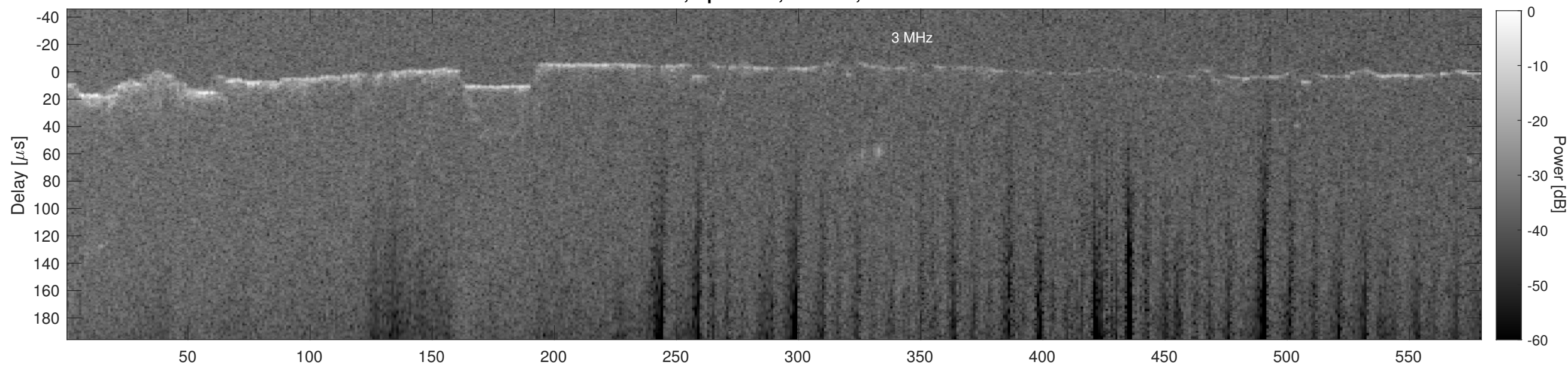
Orbit 4857, Cluttergram
