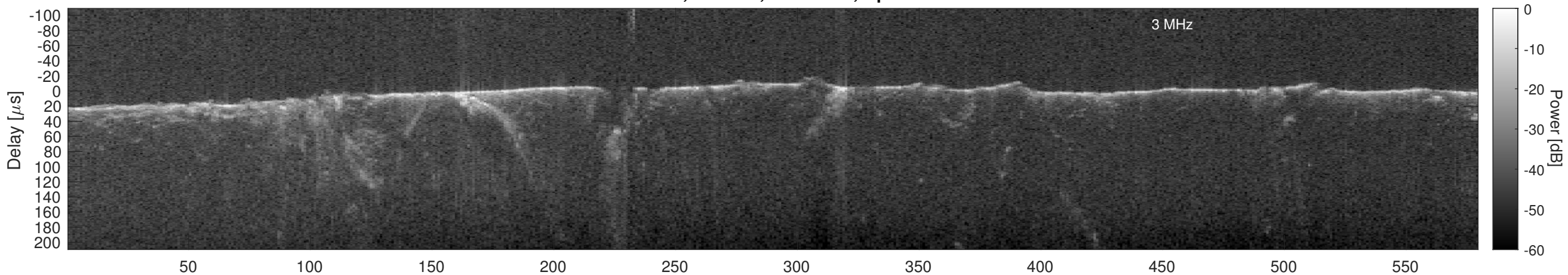
Orbit 4858, Cluttergram
