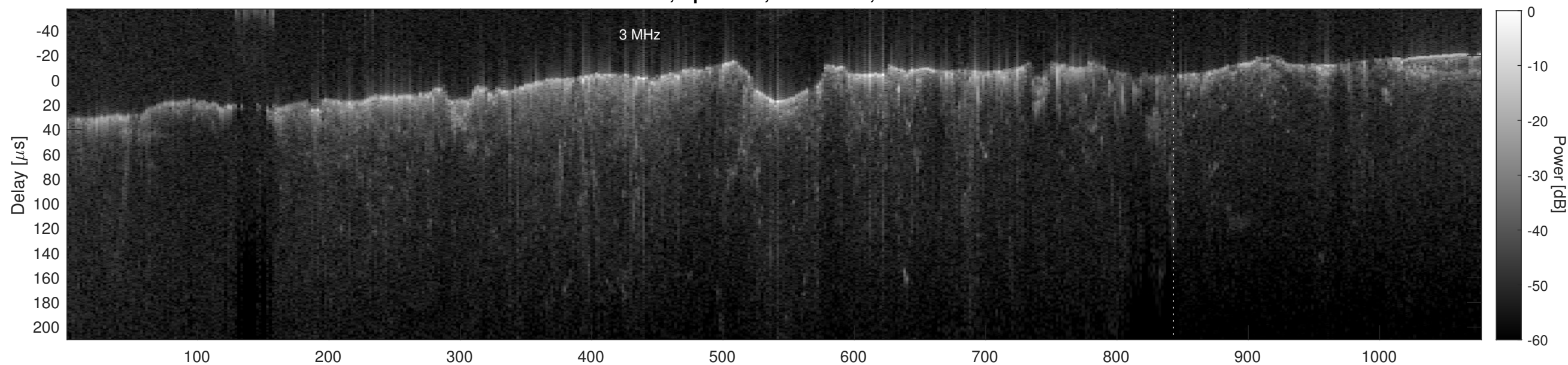
Orbit 4859, Cluttergram
