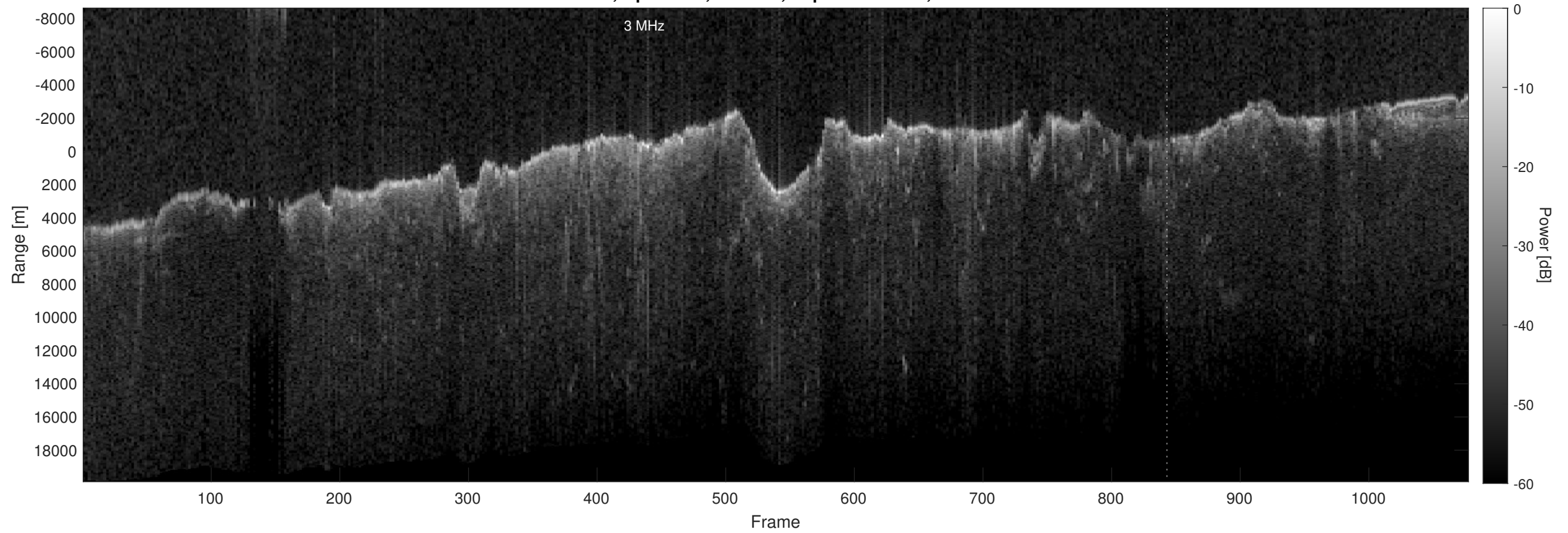
Orbit 4859, Optimized, Window, Depth-Corrected, Channel 2
