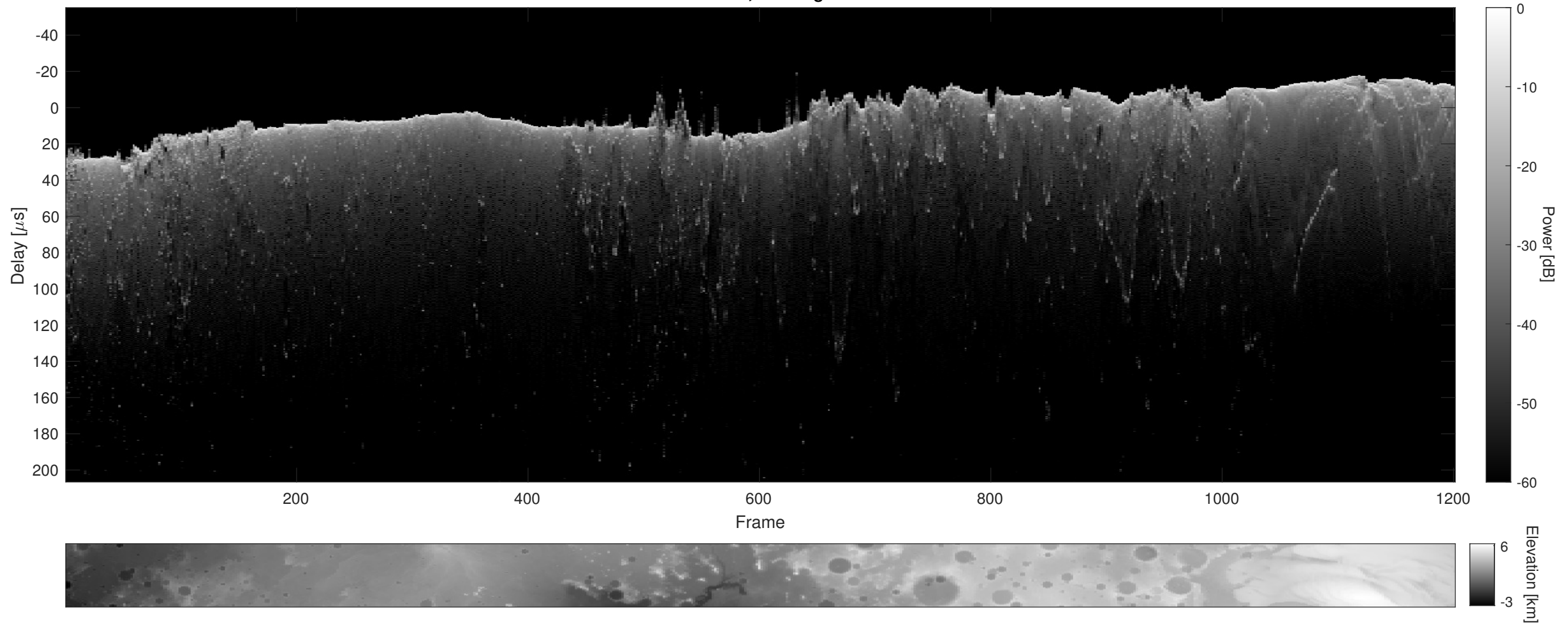
Orbit 4860, Cluttergram
