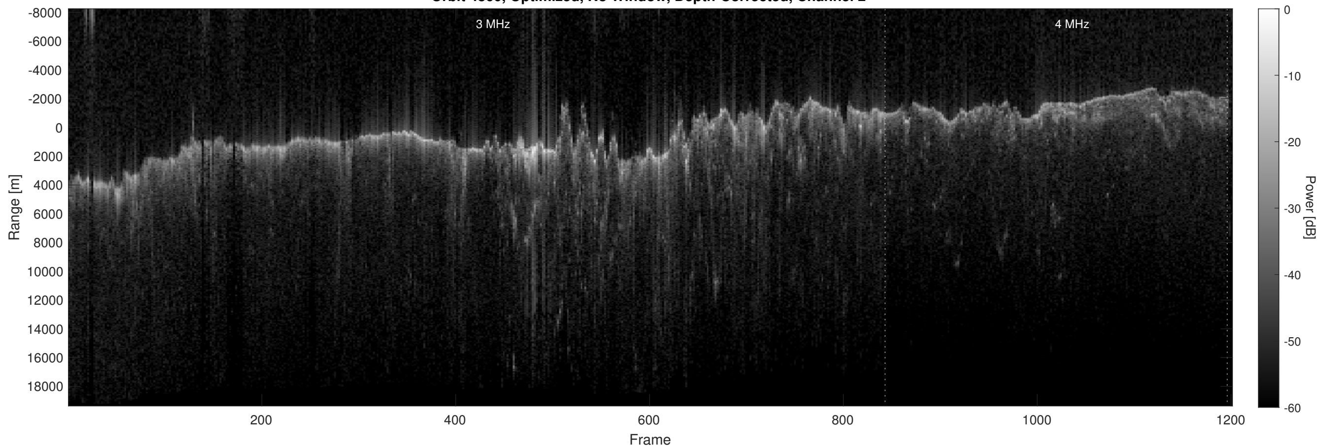
Orbit 4860, Optimized, No Window, Depth-Corrected, Channel 2
