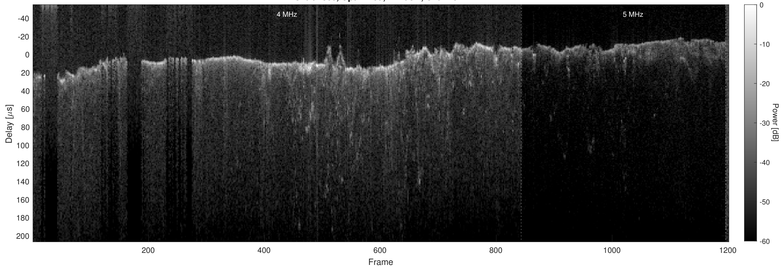
Orbit 4860, Optimized, Window, Channel 2
