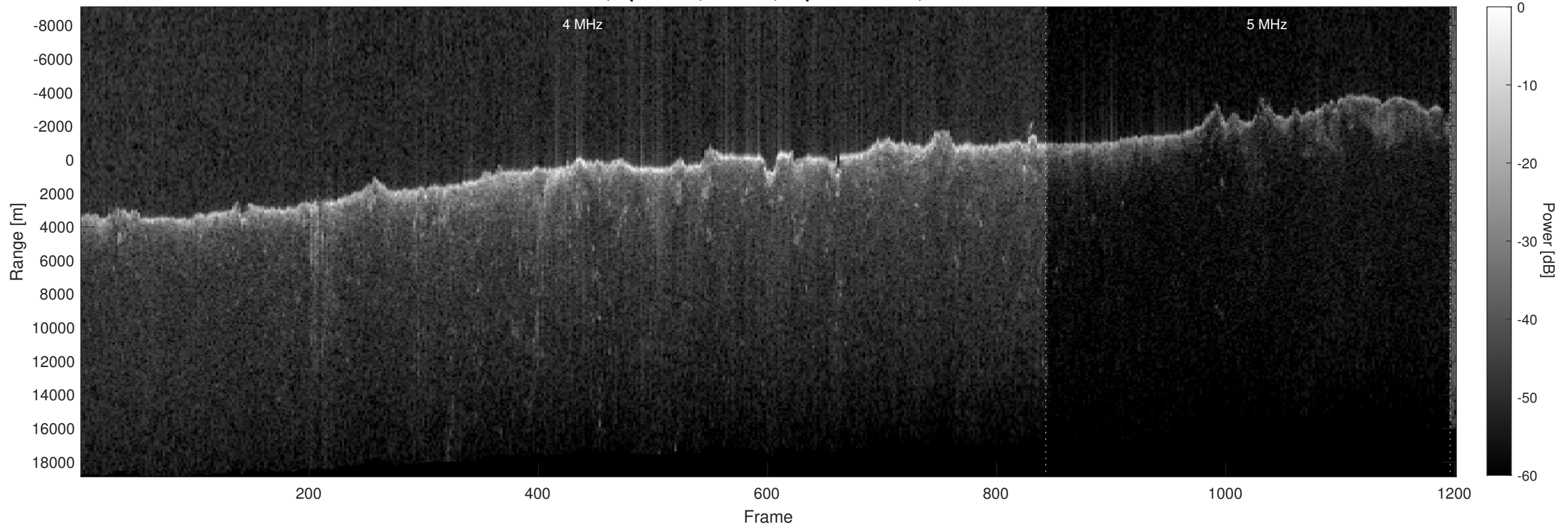
Orbit 4861, Optimized, Window, Depth-Corrected, Channel 2
