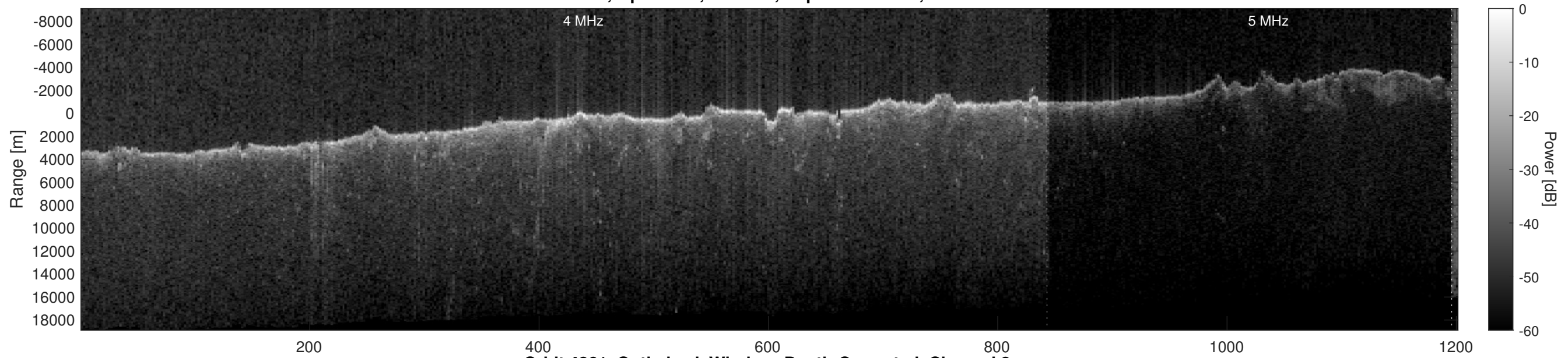
Orbit 4861, Optimized, Window, Depth-Corrected, Channel 2
