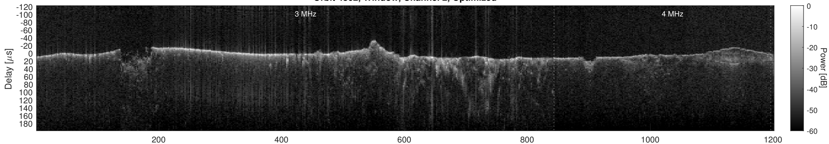
Orbit 4862, Cluttergram
