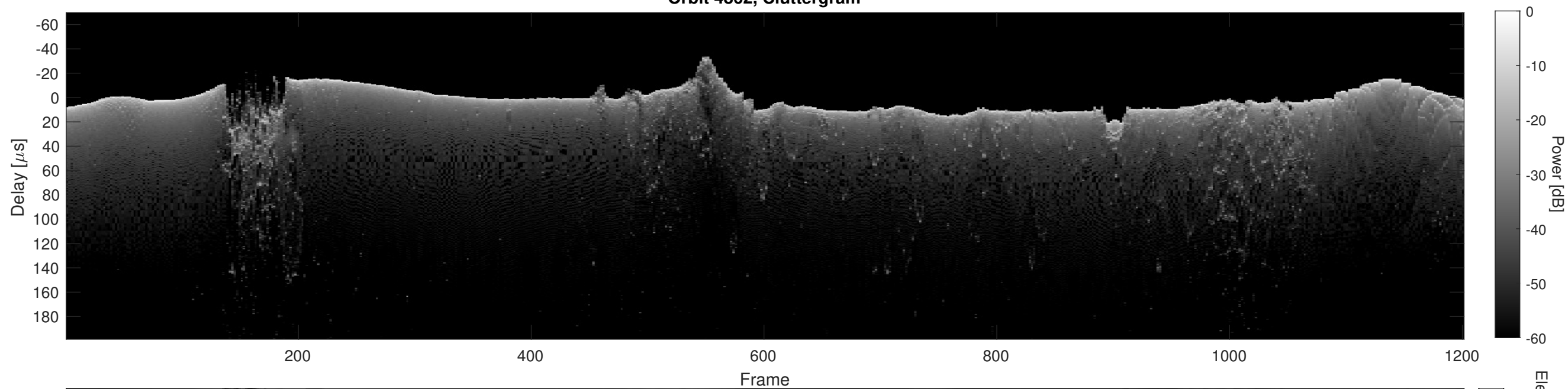
Orbit 4862, Cluttergram
