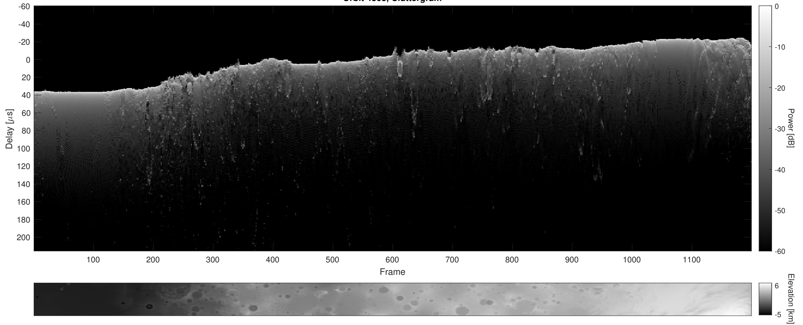
Orbit 4863, Cluttergram
