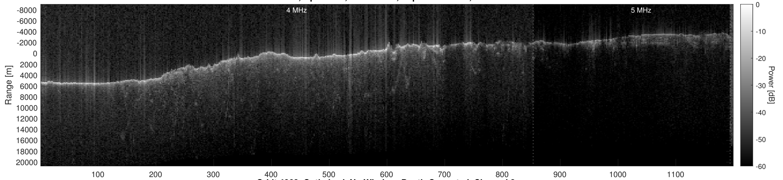
Orbit 4863, Optimized, No Window, Depth-Corrected, Channel 2
