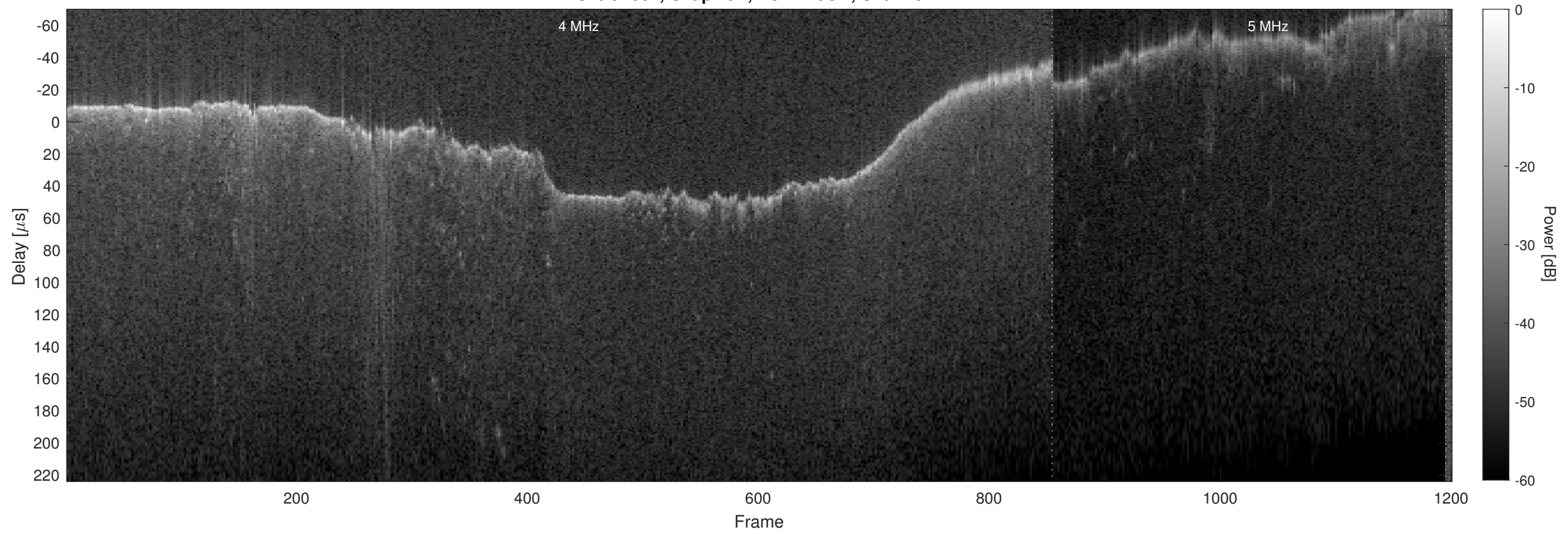
Orbit 4864, Chapman, No Window, Channel 2
