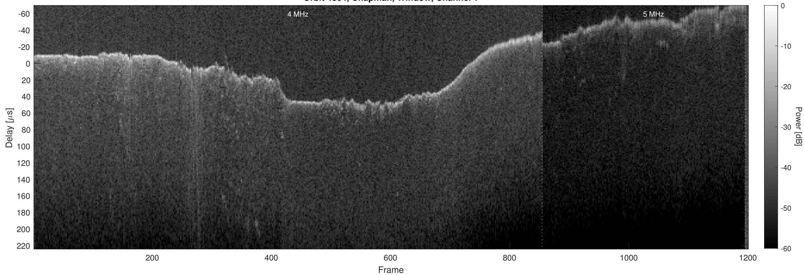
Orbit 4864, Chapman, Window, Channel 2
