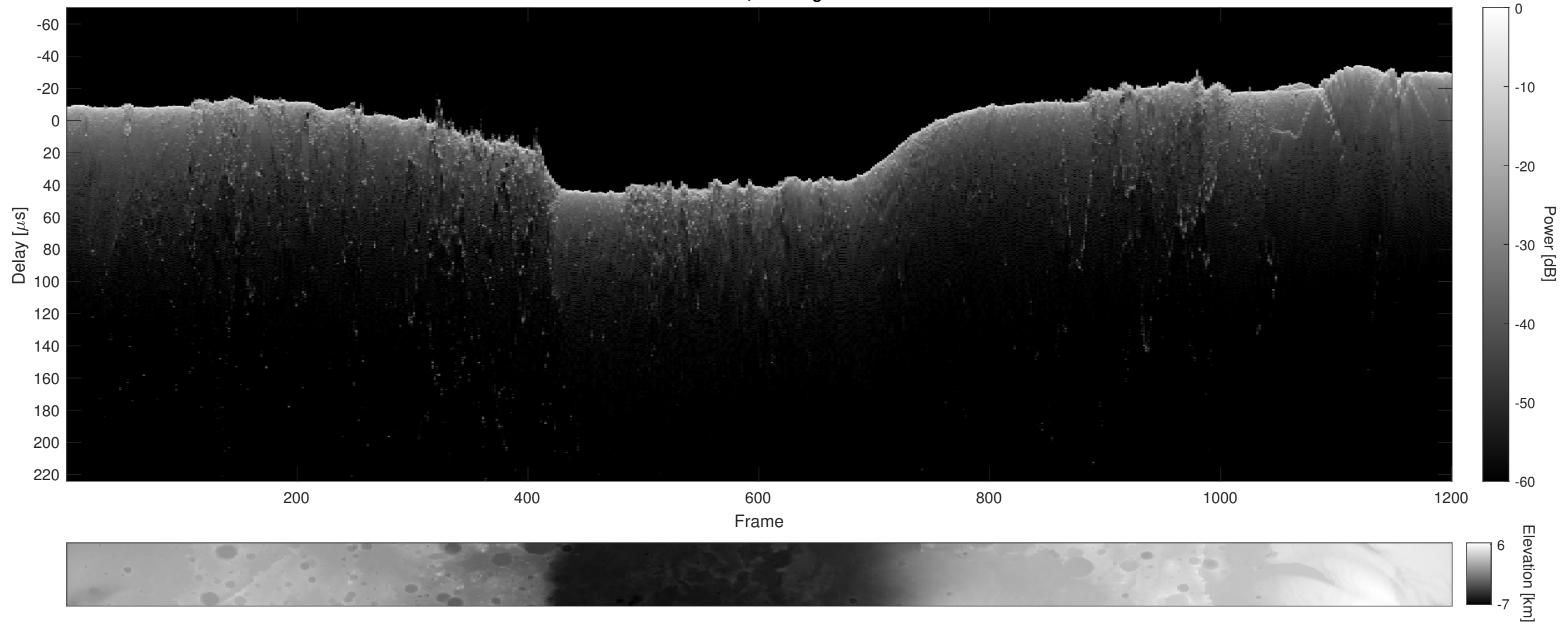
Orbit 4864, Cluttergram
