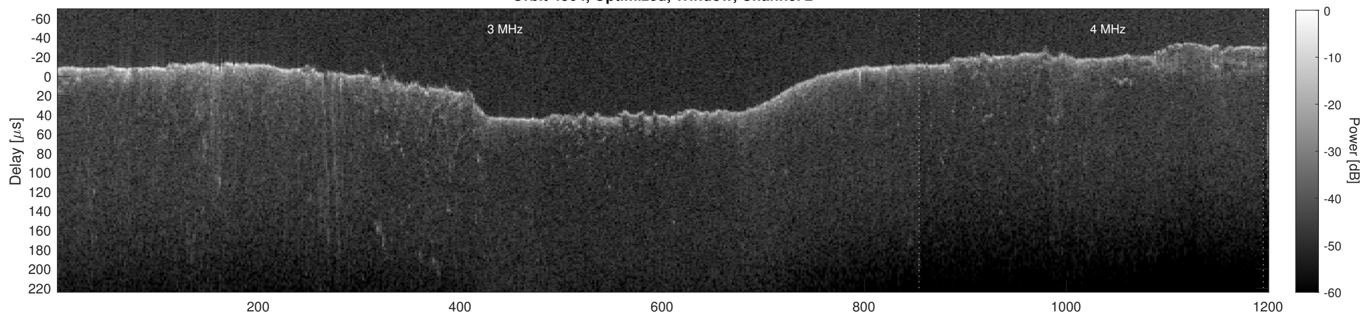
Orbit 4864, Cluttergram
