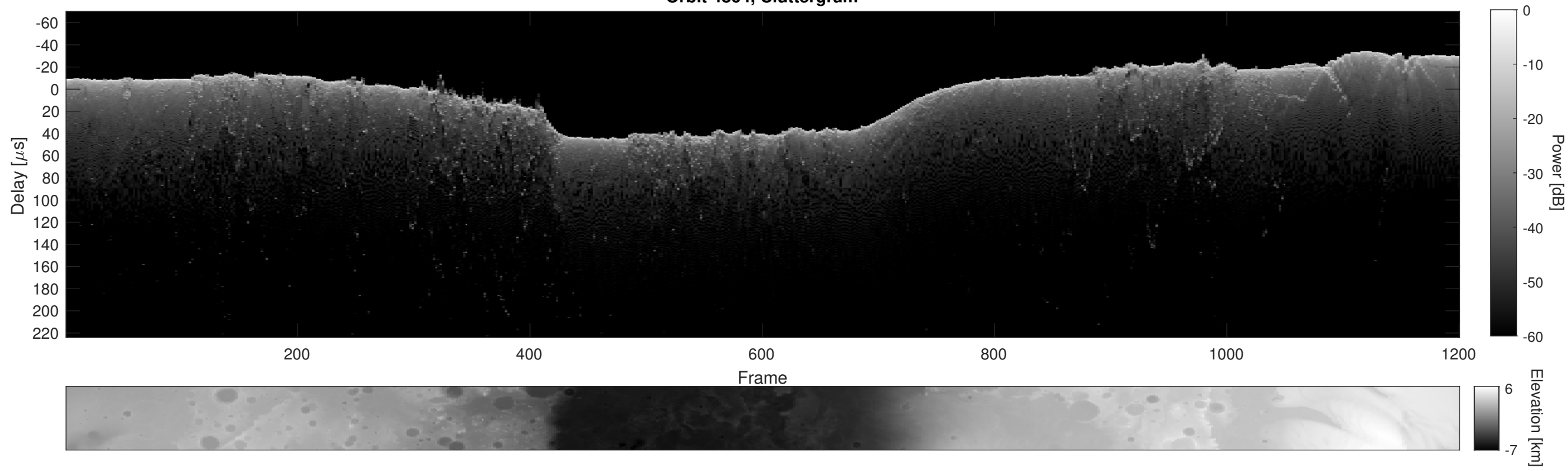
Orbit 4864, Cluttergram
