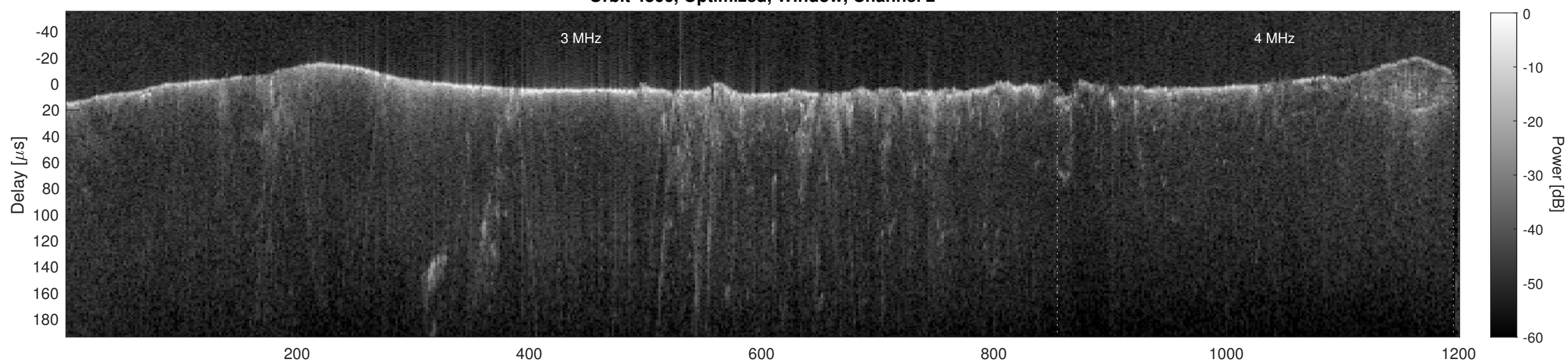
Orbit 4866, Cluttergram
