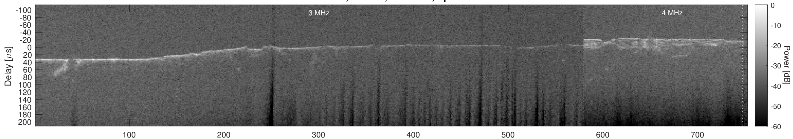
Orbit 4867, Cluttergram
