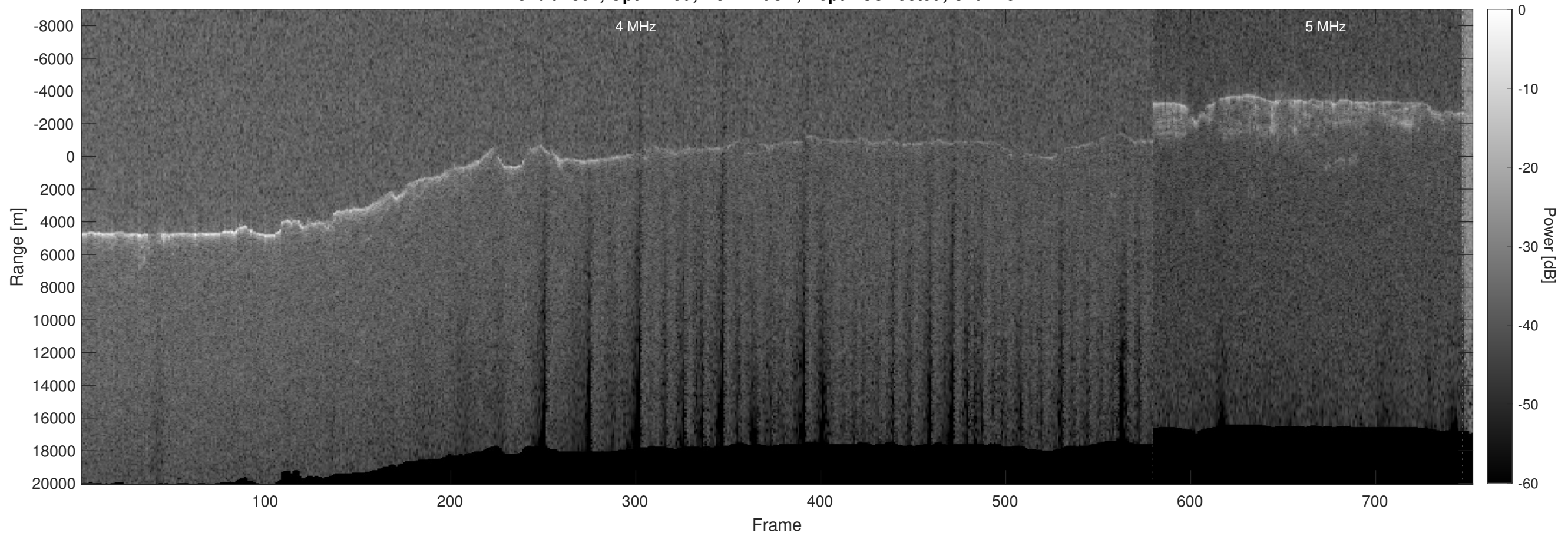
Orbit 4867, Optimized, No Window, Depth-Corrected, Channel 2
