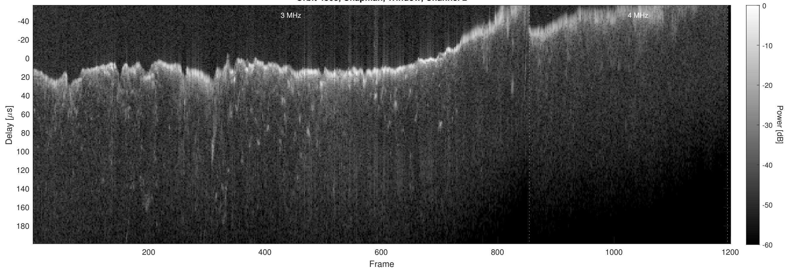
Orbit 4868, Chapman, Window, Channel 2
