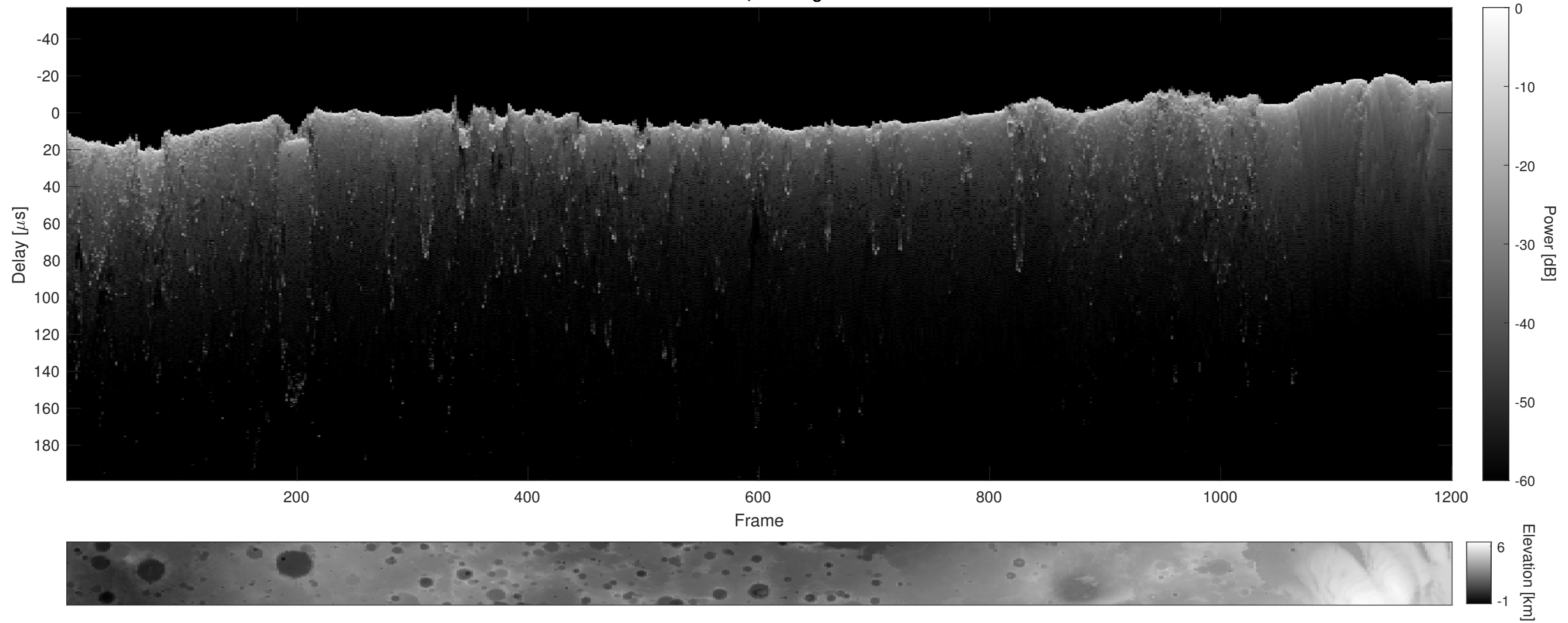
Orbit 4868, Cluttergram
