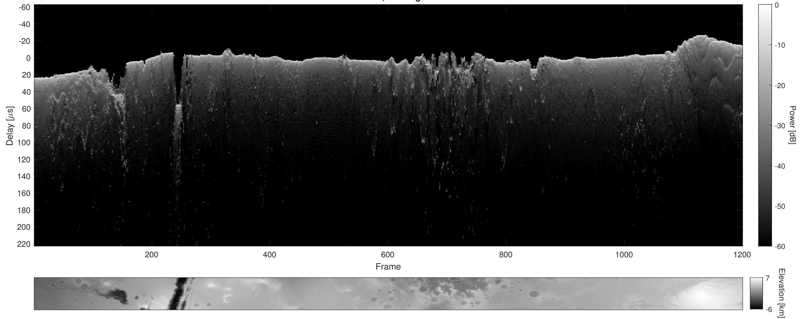
Orbit 4869, Cluttergram
