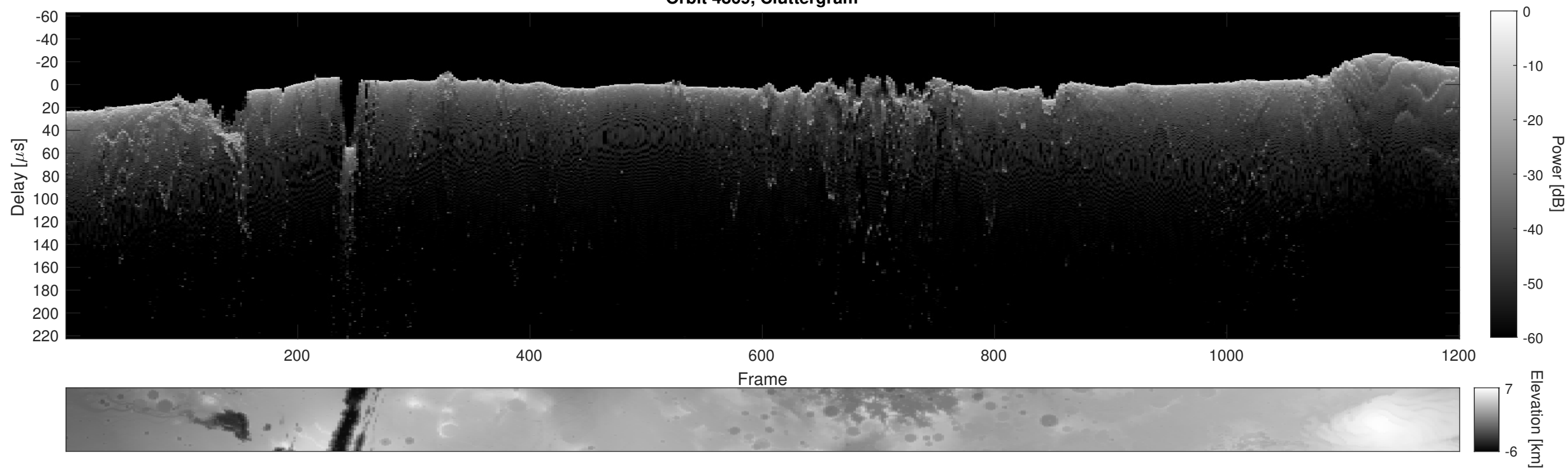
Orbit 4869, Cluttergram
