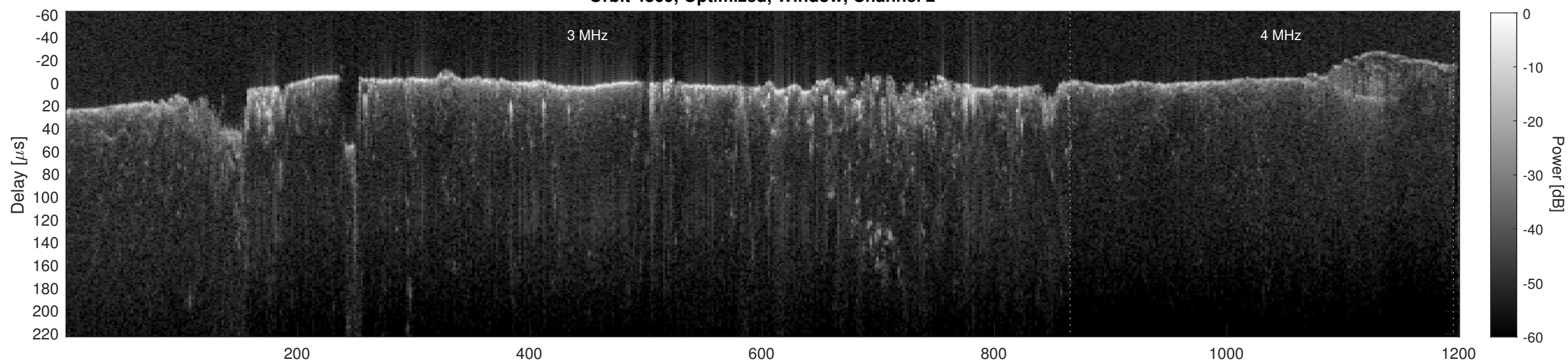
Orbit 4869, Cluttergram
