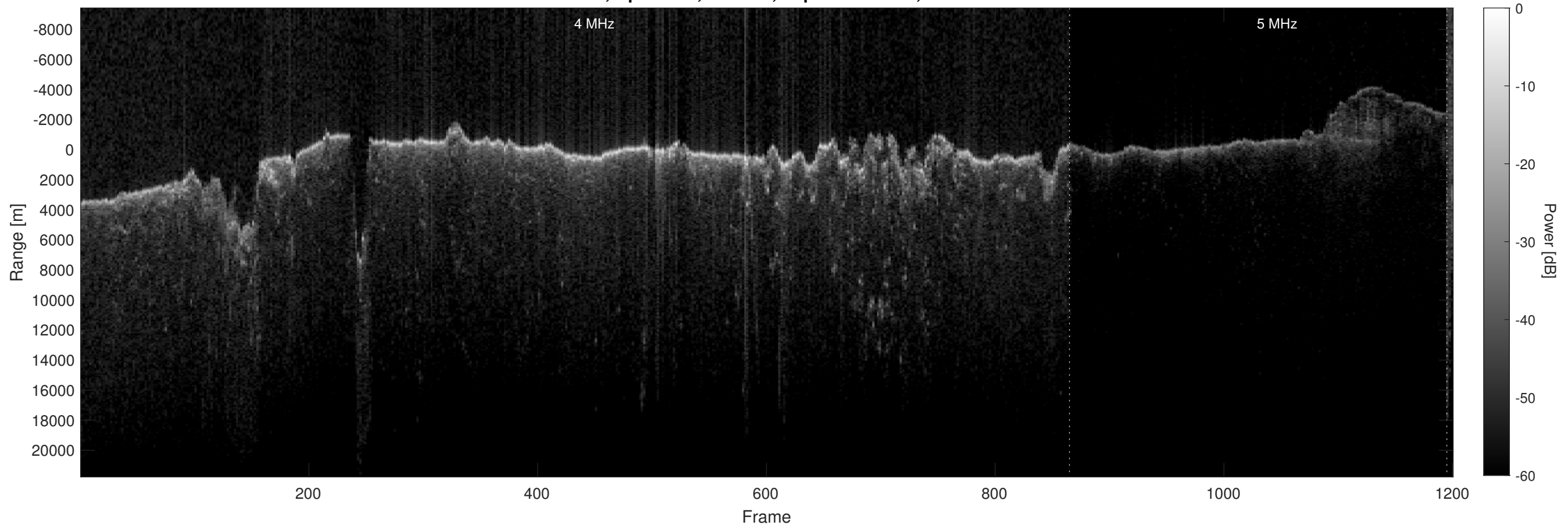
Orbit 4869, Optimized, Window, Depth-Corrected, Channel 2
