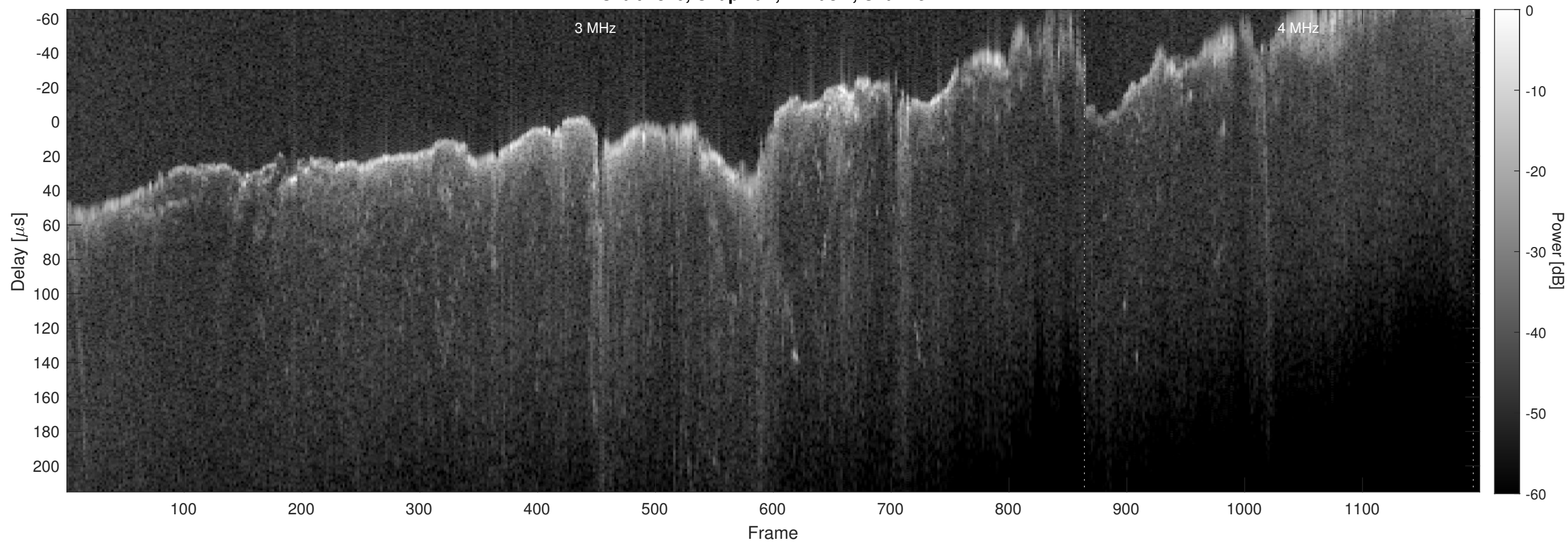
Orbit 4870, Chapman, Window, Channel 2
