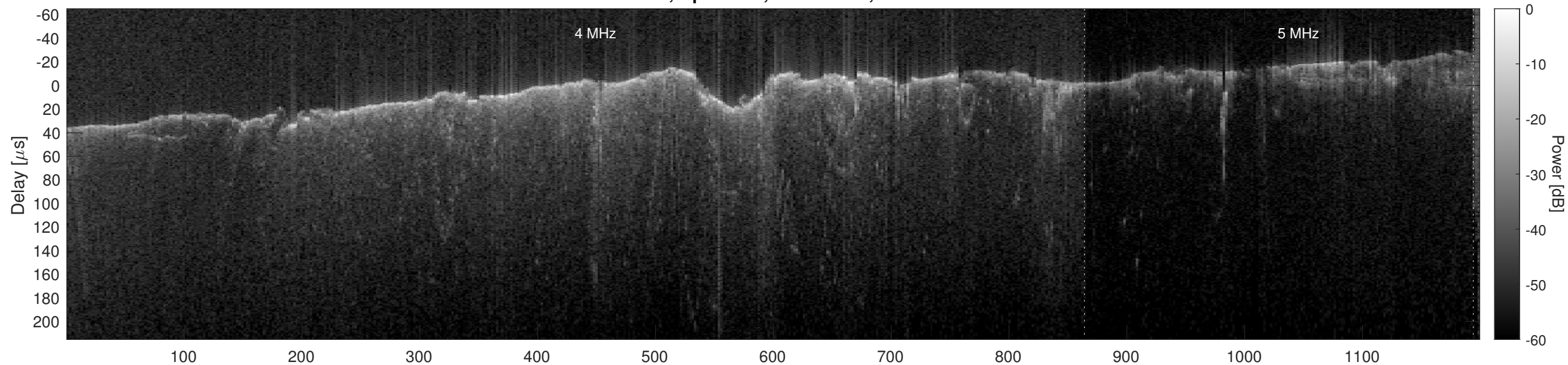
Orbit 4870, Optimized, No Window, Channel 2
