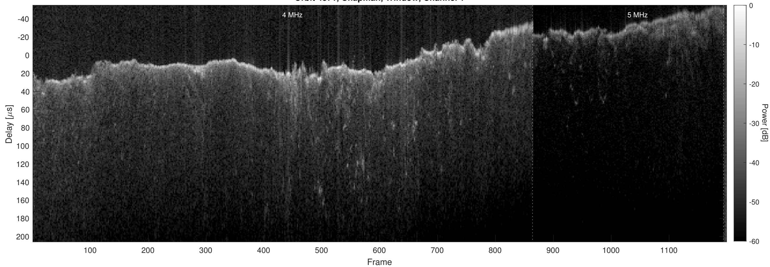
Orbit 4871, Chapman, Window, Channel 2
