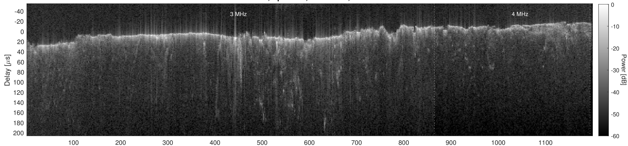
Orbit 4871, Cluttergram
