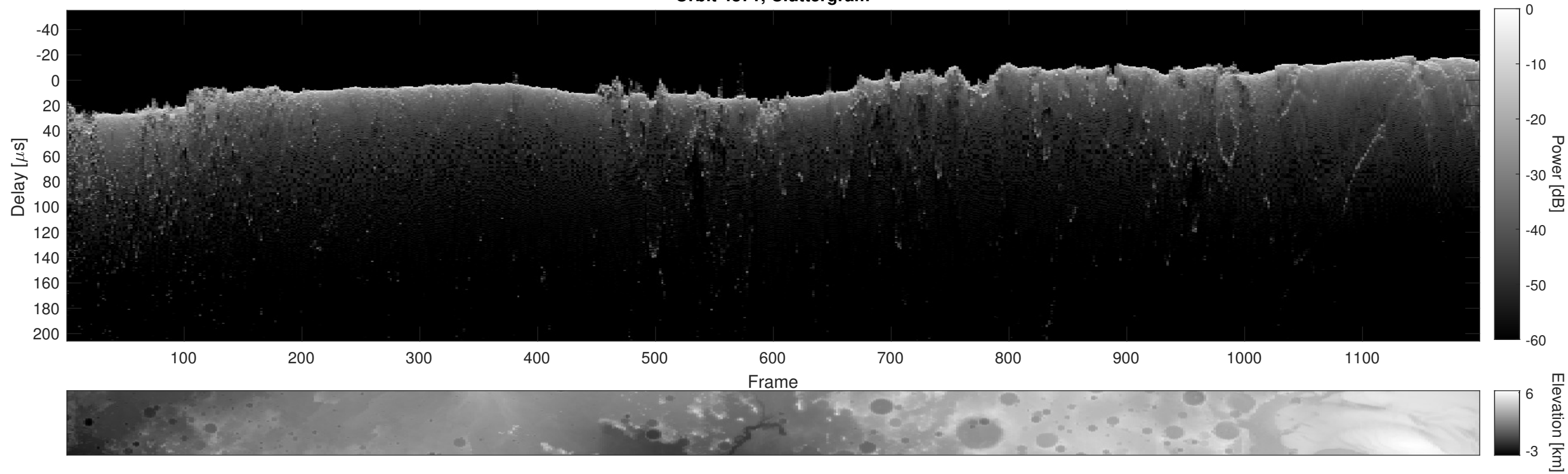
Orbit 4871, Cluttergram
