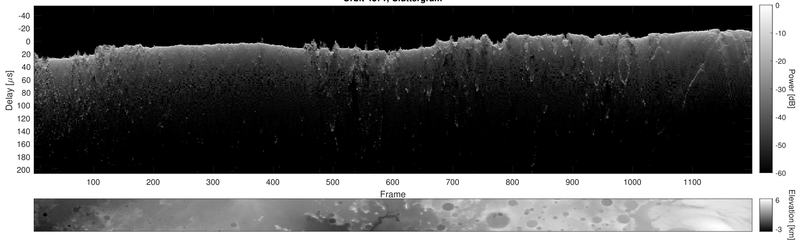
Orbit 4871, Cluttergram
