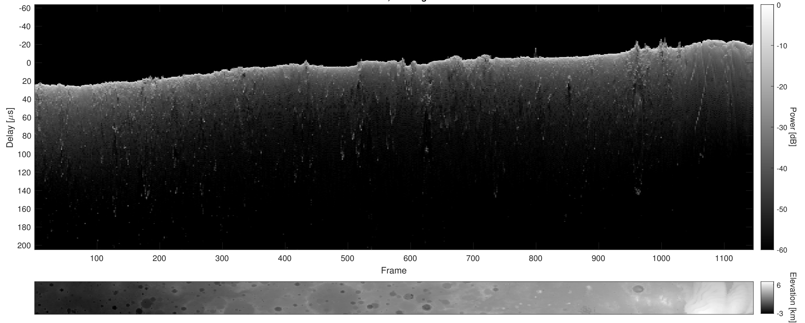
Orbit 4872, Cluttergram
