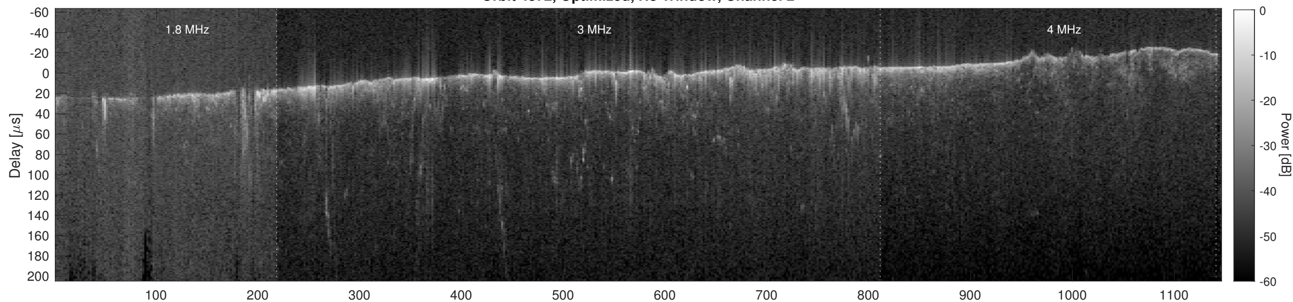
Orbit 4872, Cluttergram
