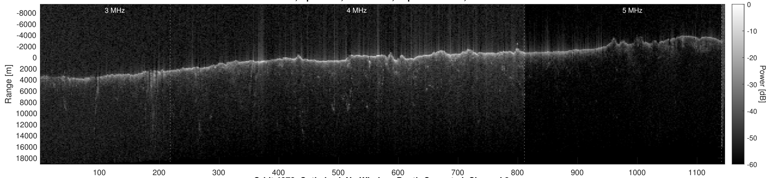
Orbit 4872, Optimized, No Window, Depth-Corrected, Channel 2
