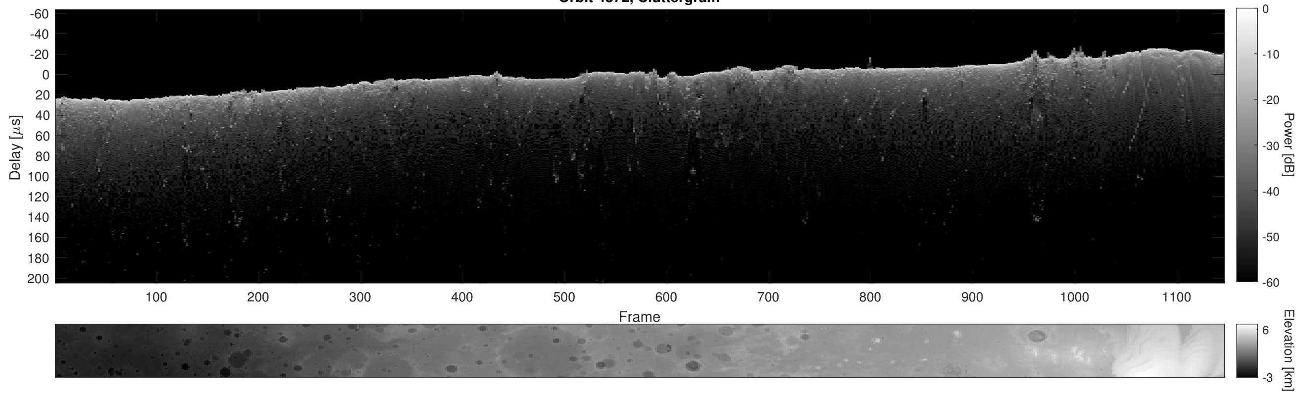
Orbit 4872, Cluttergram
