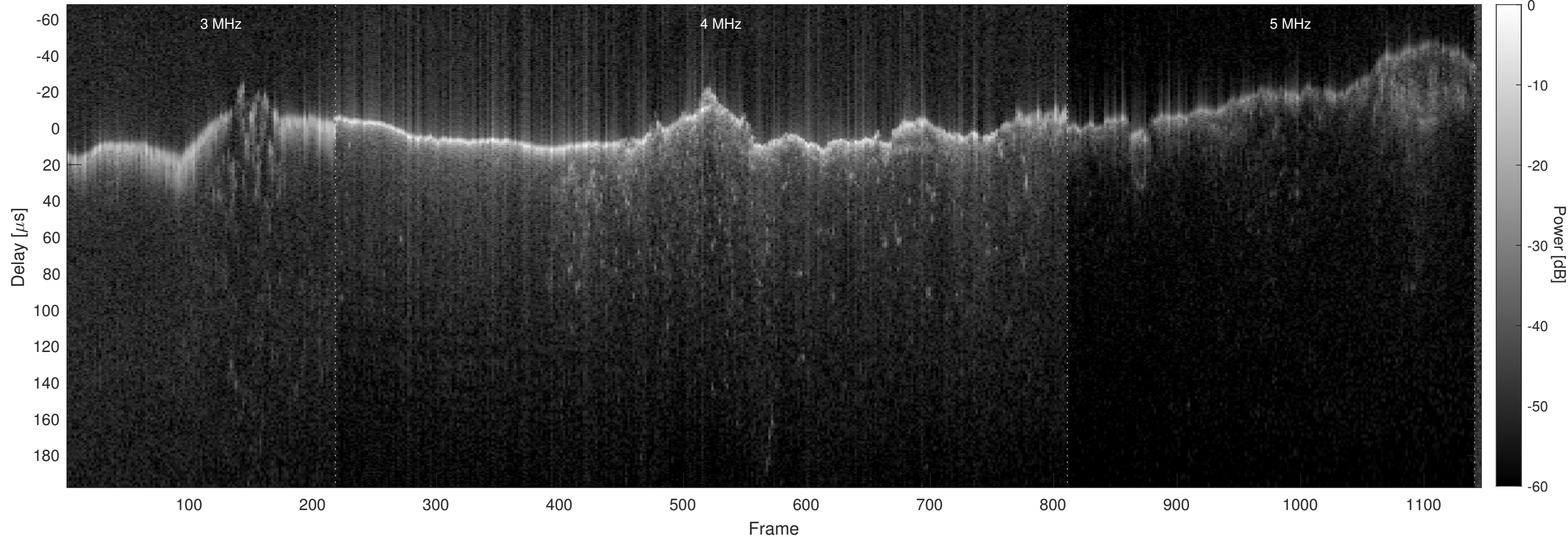
Orbit 4873, Chapman, No Window, Channel 2
