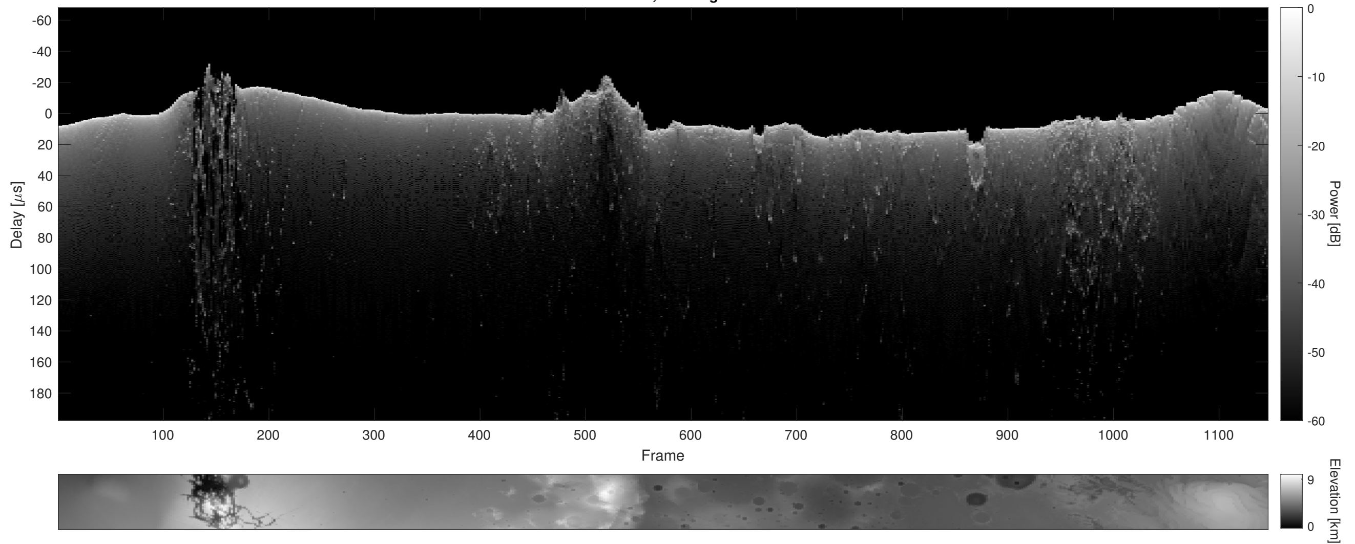
Orbit 4873, Cluttergram
