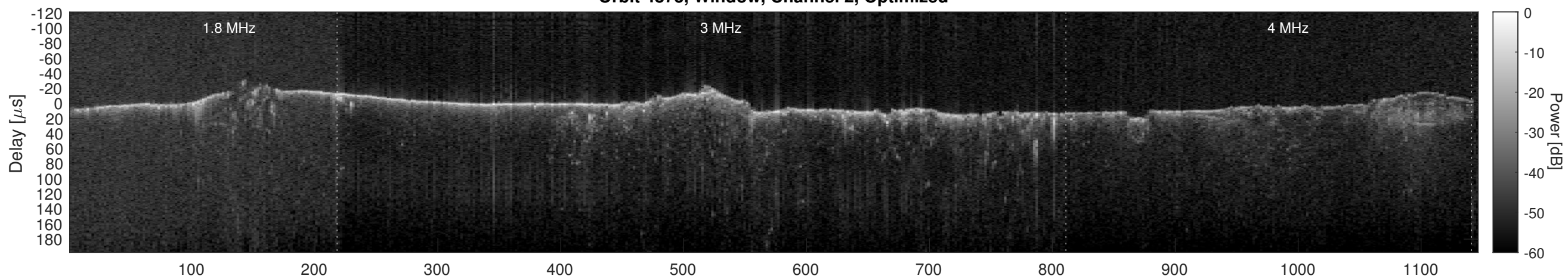
Orbit 4873, Cluttergram
