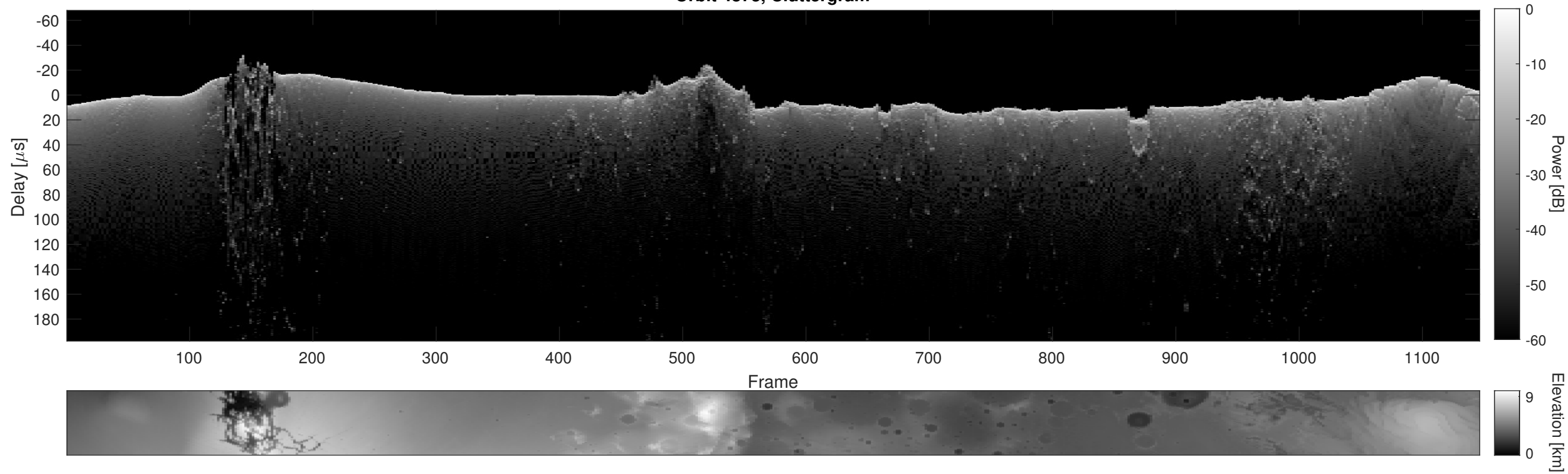
Orbit 4873, Cluttergram
