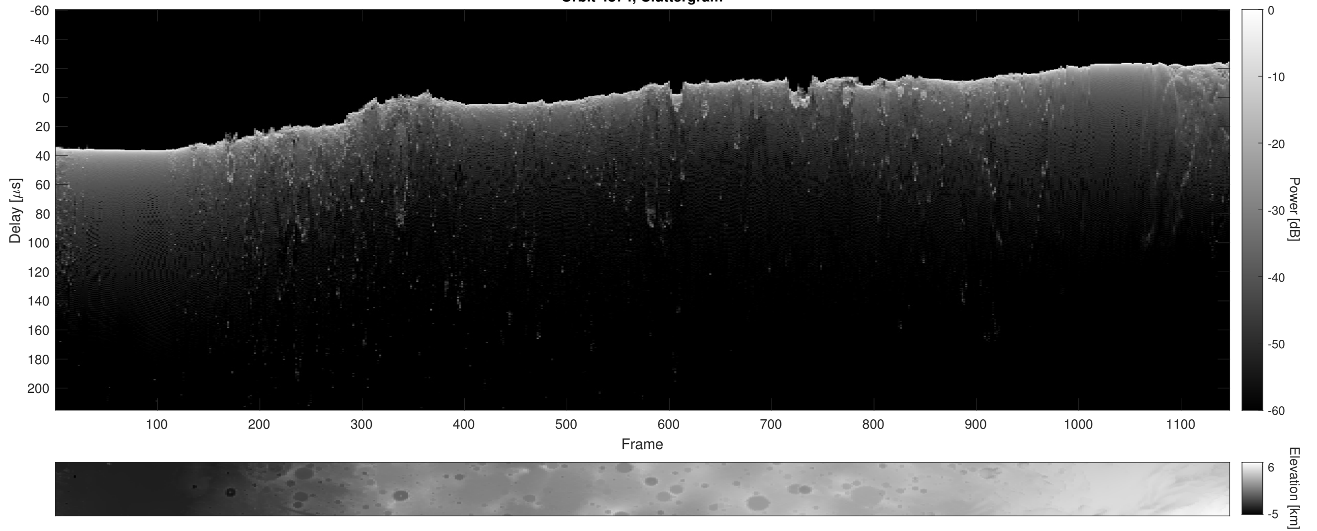
Orbit 4874, Cluttergram
